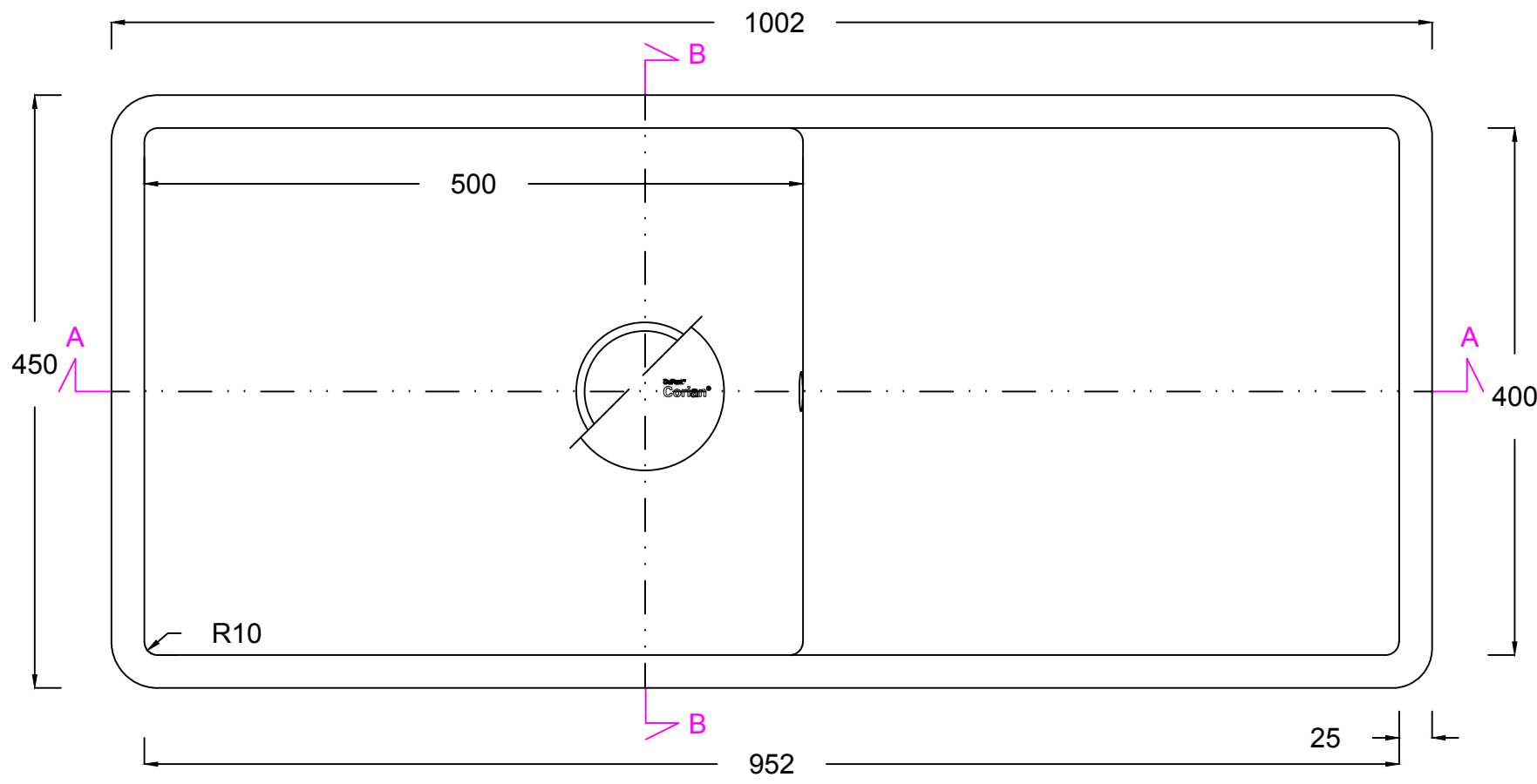
PLAN VIEW
