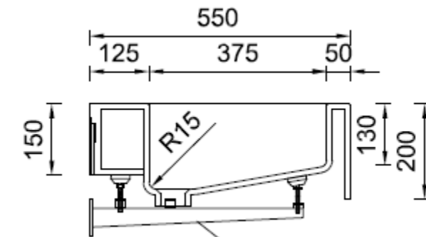
cantilever wall brackets
